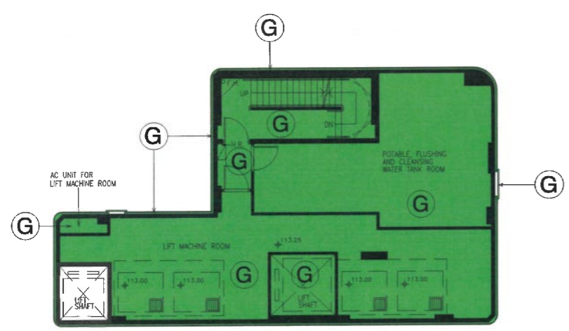
TOWER 2 - LIFT MACHINE ROOM PLAN
