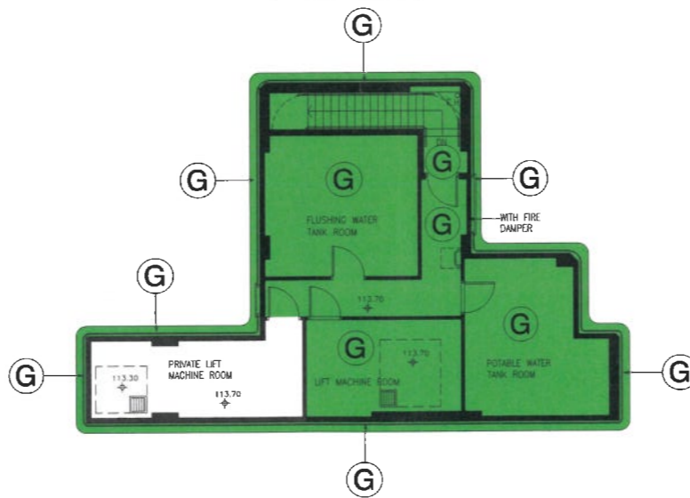
UPPER ROOF PLAN
