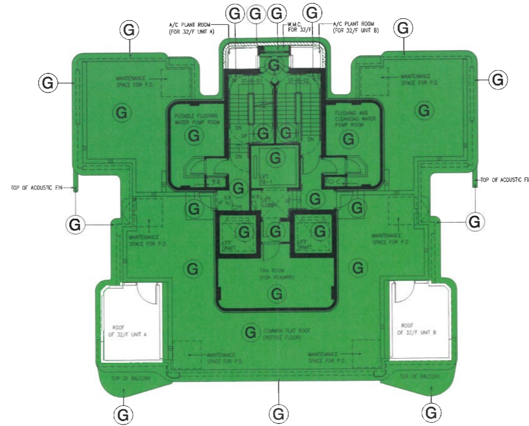
ROOF PLAN
